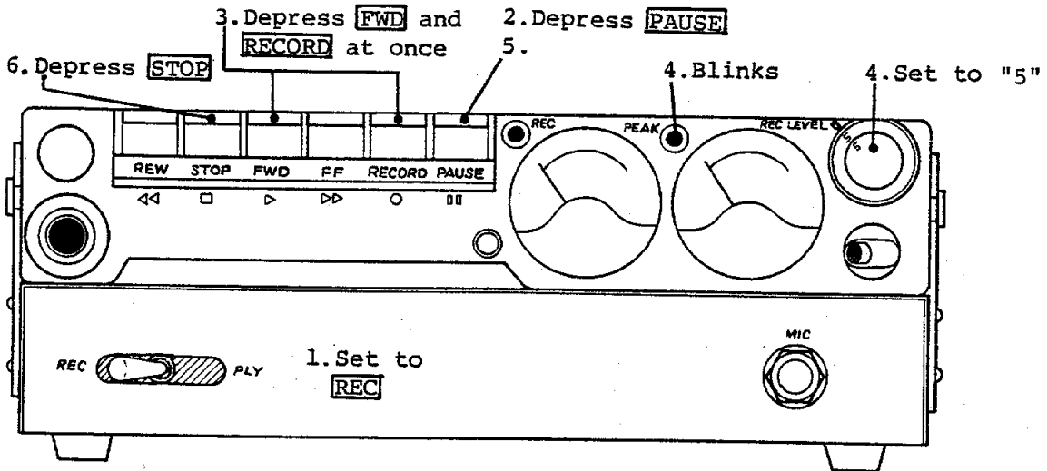
Fig. 2 Recording Procedure
